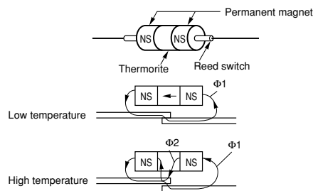
(b) Normally open type
