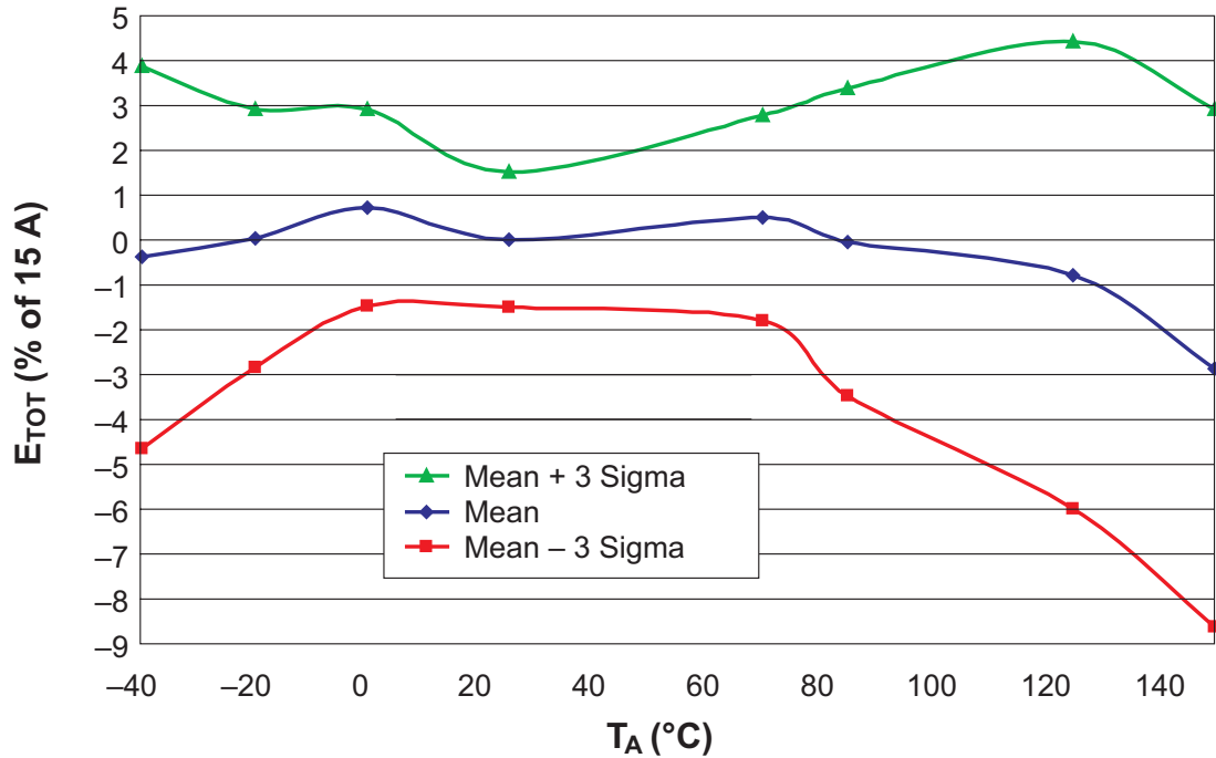
Typical Percentage Error versus Ambient Temperature Measurements at T_A = -40, -20, 0, 25, 70, 85, 125, and 150\text{ }^\circ\text{C}
