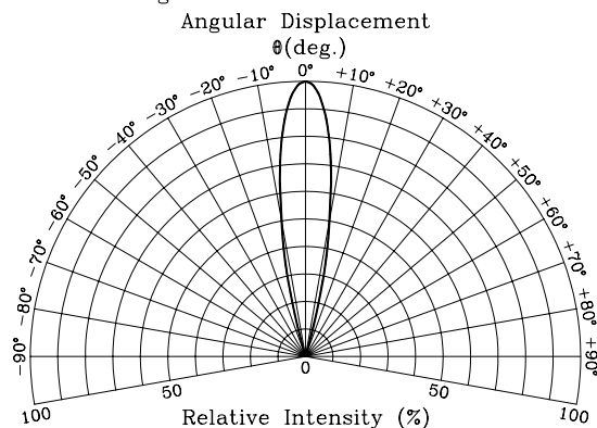
Radiation Diagram
