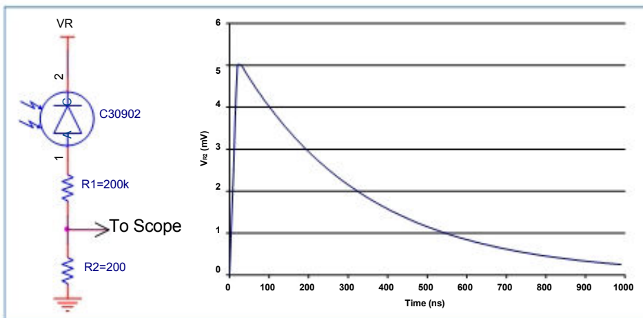
Figure 14 Sample of passive quench circuit
