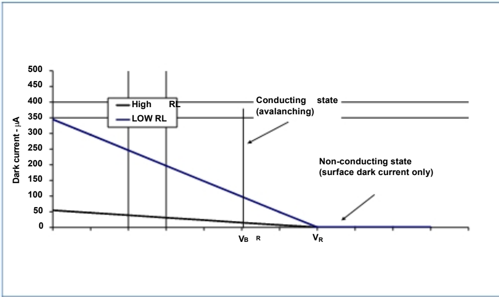
Figure 8 Load Line for C30921SH in the Geiger mode
