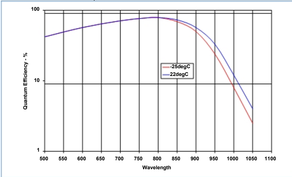
Figure 2 Typical quantum efficiency vs. wavelength
