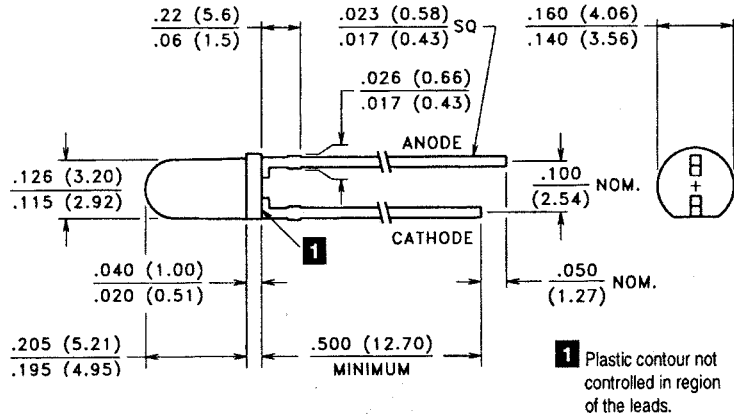
CASE 50A Long T-1 (3 mm) CHIP SIZE: .011" x .011"
