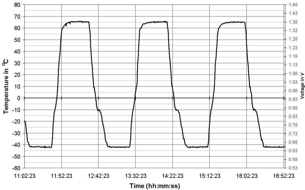
3 Sampled (Normalized Offset Voltage) Temperature Cycles
