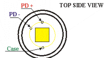
Package TO-5
