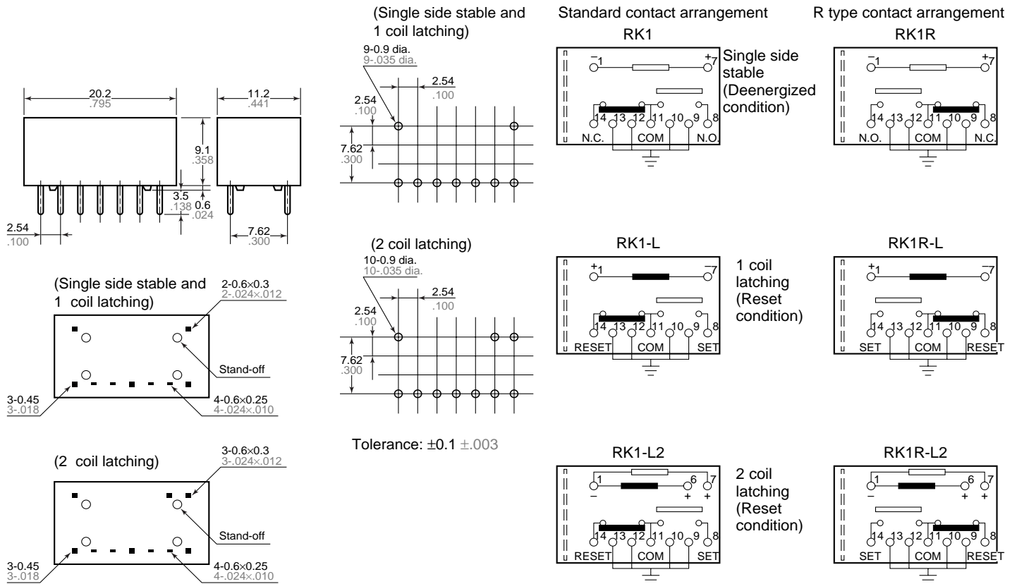
PC board pattern (Copper-side view)
