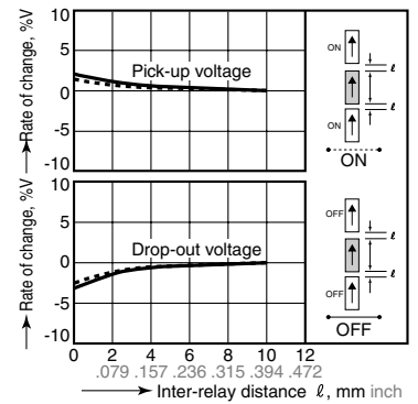
9-(2). Influence of adjacent mounting Tested sample: AGQ20012, 6 pcs.
