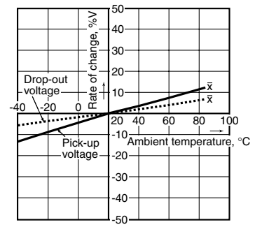
7. Ambient temperature characteristics Tested sample: AGQ2004H, 6 pcs.
