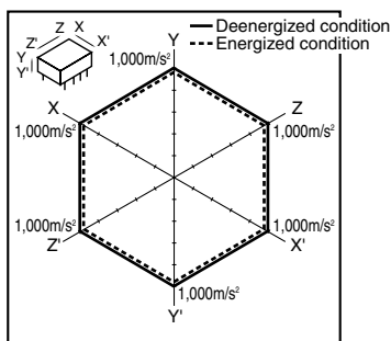
8. Malfunctional shock Tested sample: AGQ2004H, 6 pcs.
