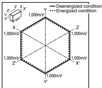
8. Malfunctional shock Tested sample: AGN2004H
