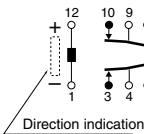
1 coil latching
