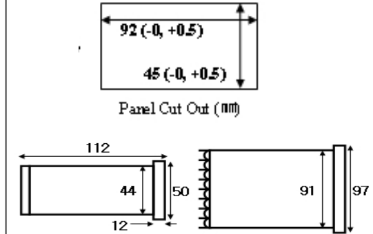
Fig. 2 Size of UV Radiometer 5.0
