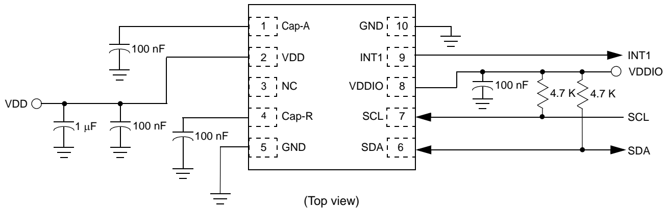
Figure 4. Electrical connection
