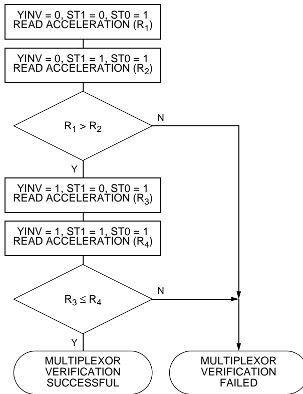
Figure 2-2 DSP Input Multiplexer Verification Flow Chart (Y Axis)
