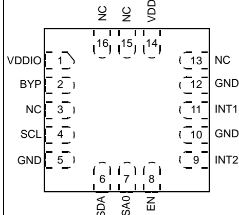
Pin Connections
