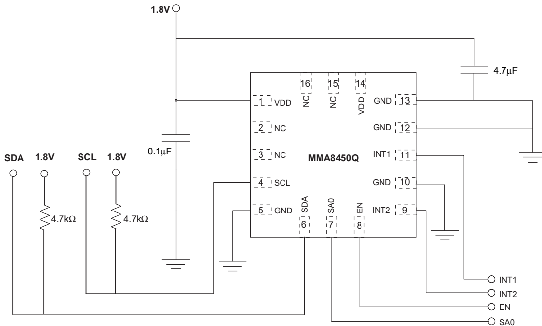
Figure 4. Application Diagram
