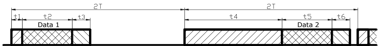
Extended PWM Output Format
