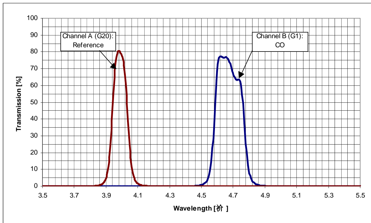
Fig.4: Filter Transmission
