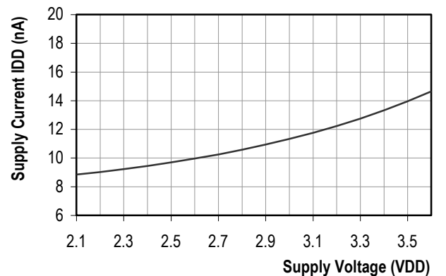
Figure 7 Typical dependency of supply current (sleep mode) versus supply voltage at 25°C. Please note the variance of the displayed data may exceed ±25%.
