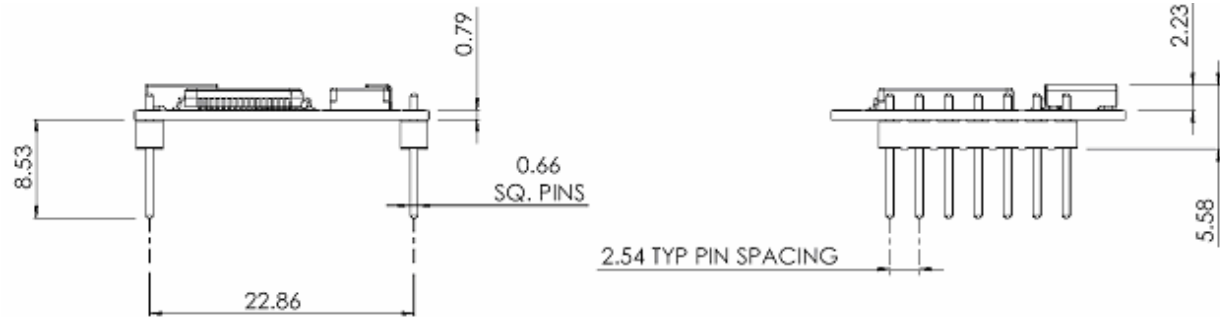
Figure 3: Side Views
