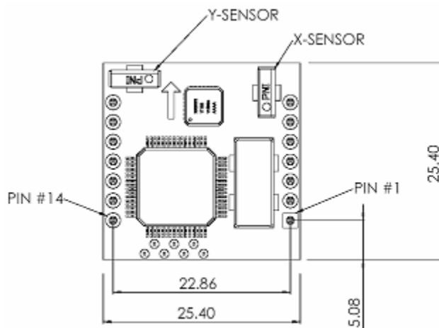
Figure 4: Top View
