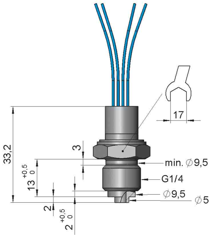
Scale Drawing C- and T-Types
