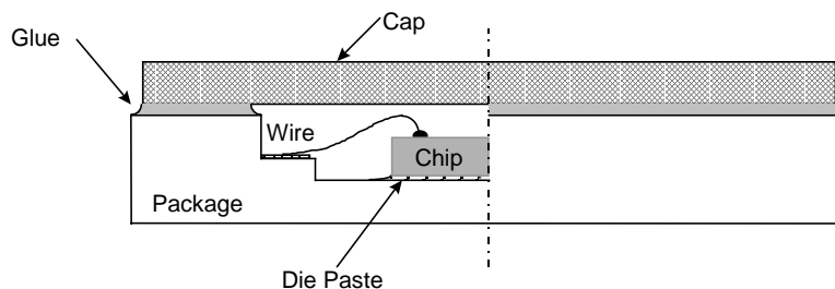
Cross-section of MBF9042BB
