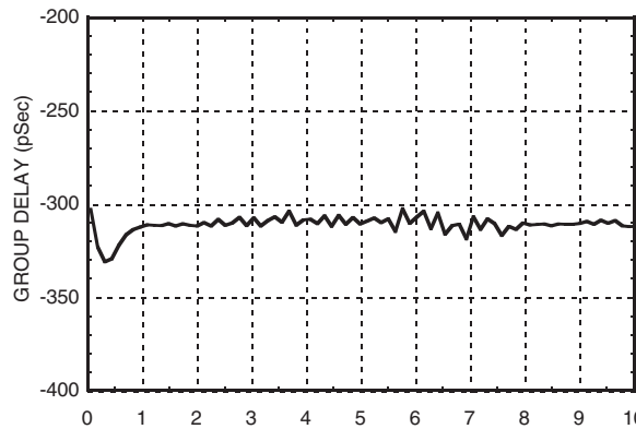
Group Delay
