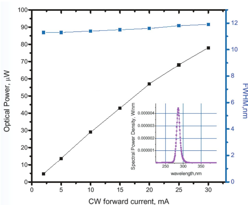
LI curve on 290nm fiber coupled device
