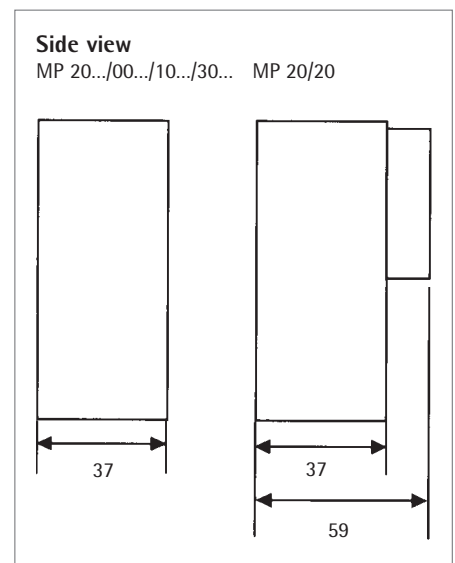
MP 20/30 four LC junction unit
