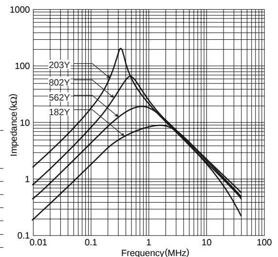
TYPICAL ELECTRICAL CHARACTERISTICS IMPEDANCE vs. FREQUENCY CHARACTERISTICS
