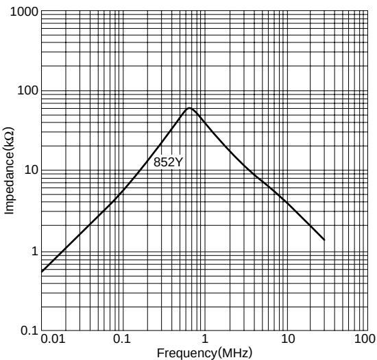
TYPICAL ELECTRICAL CHARACTERISTICS IMPEDANCE vs. FREQUENCY CHARACTERISTICS
