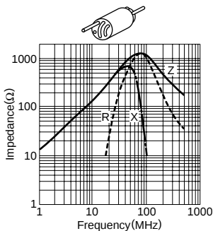
HF40R6H6X10H0.8 (5 holes)
