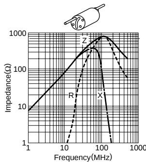
HF40R6H6X10H0.8 (3 holes)
