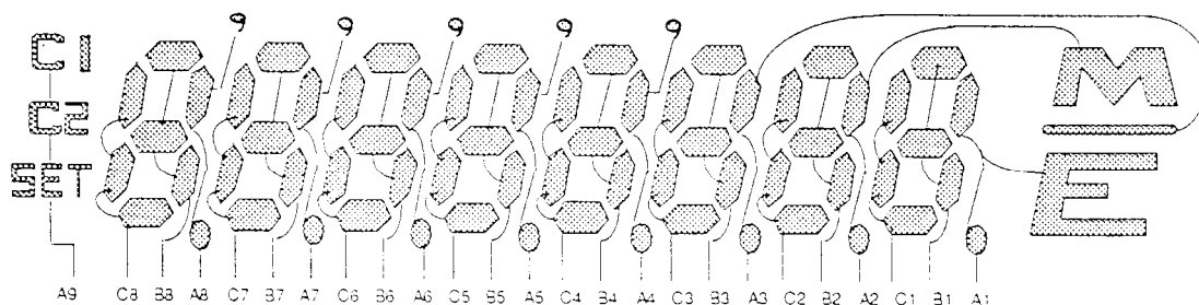
Segment Connection
