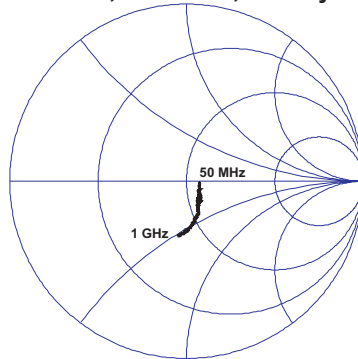
Figure 19: Unmatched Device Output Impedance S24 Packaged Device
