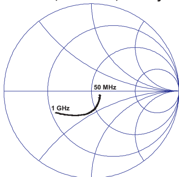
Figure 18: Unmatched Device Input Impedance S24 Packaged Device
