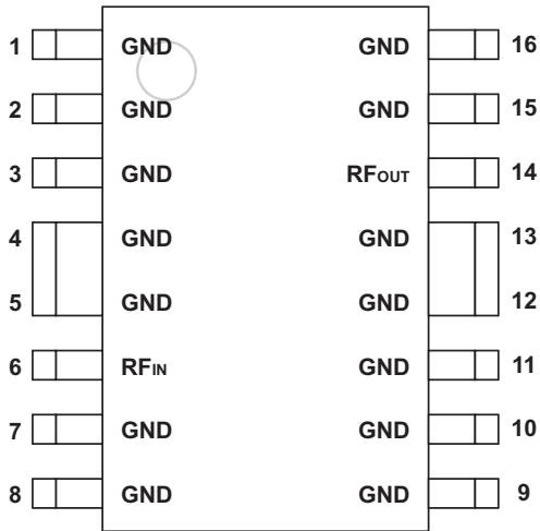
Figure 2: Pinout - S3 Package
