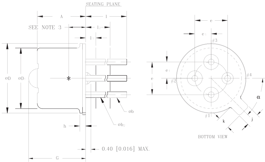
MM CONTROLLING DIMENSIONS
