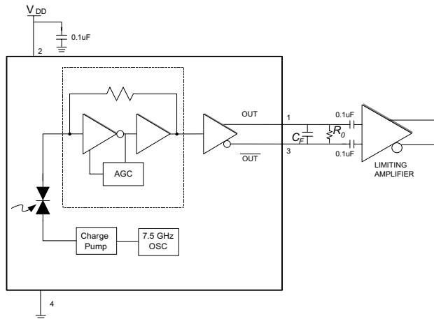
Figure 14: Application Schematic
