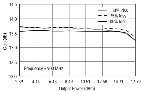
Gain vs. Power Out
