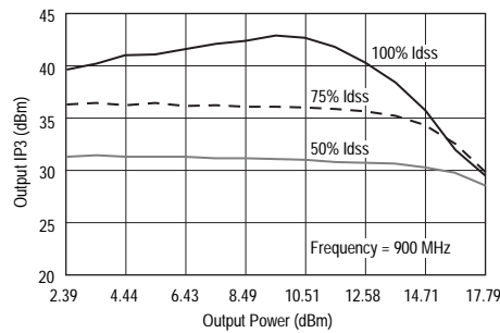
Output IP3 vs. Power Out
