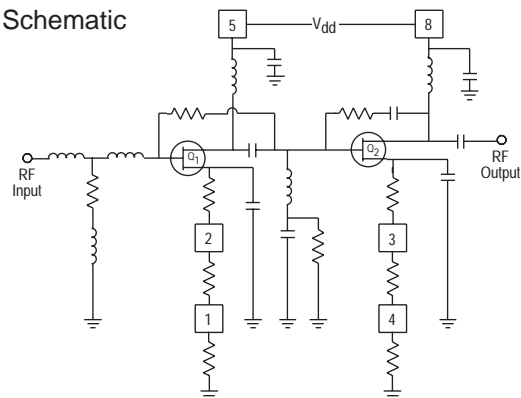
Schematic
