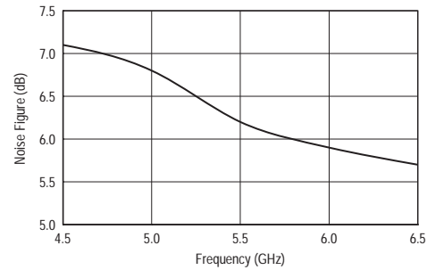
Noise Figure
