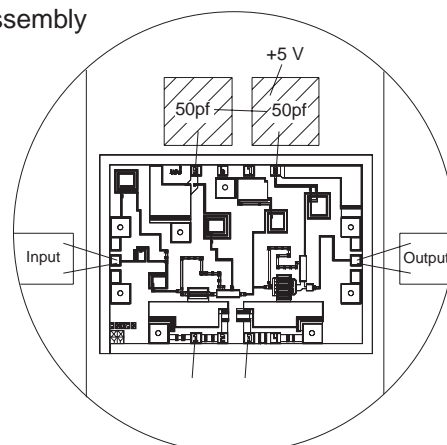
Assembly
