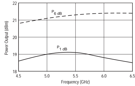
Power Output
