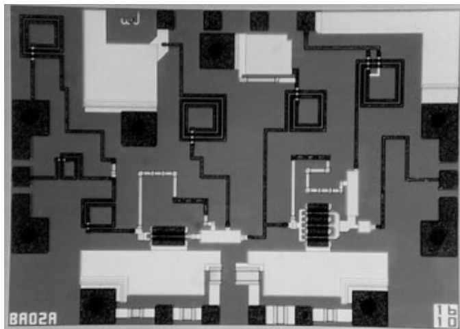
ICA1001 Chip Outline
