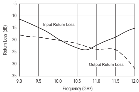
Return Loss
