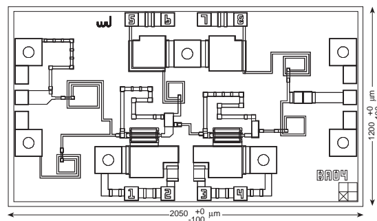
ICA1002 Chip Outline
