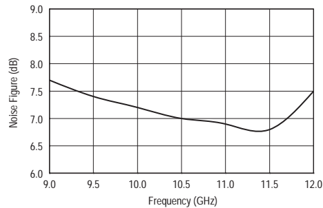
Noise Figure
