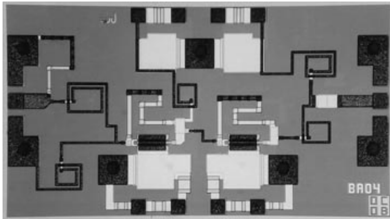
ICA1002 Chip Outline
