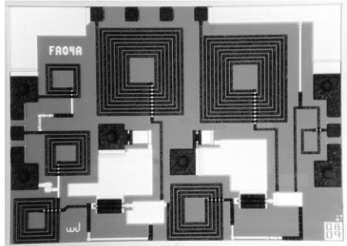
ICA1004 Chip Outline
