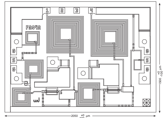
ICA1004 Chip Outline
