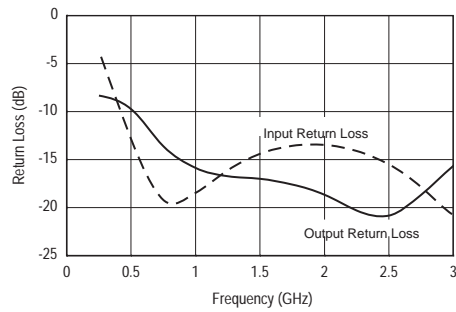
Return Loss
