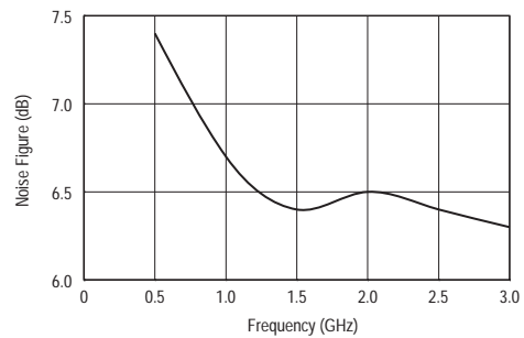
Noise Figure
