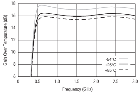
Gain Over Temperature
