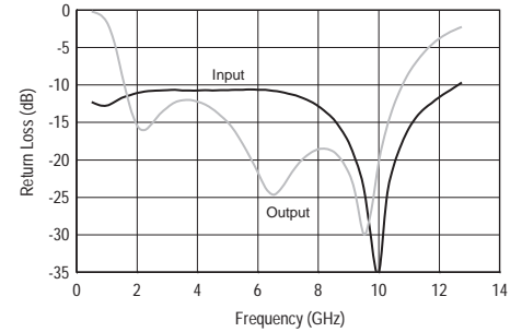
Return Loss
