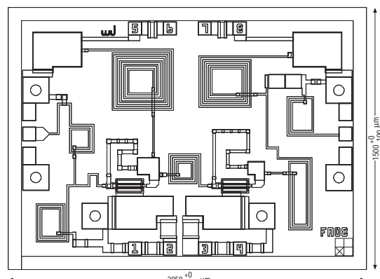
ICA1008 Chip Outline
