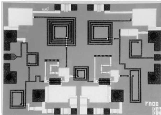
ICA1008 Chip Outline
