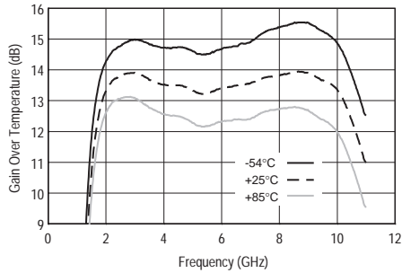
Gain Over Temperature
