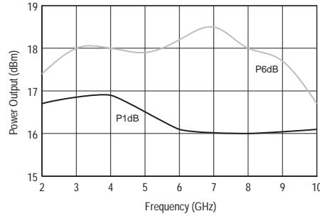
Power Output
