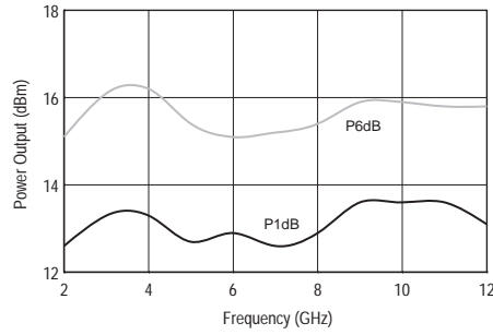
Power Output
