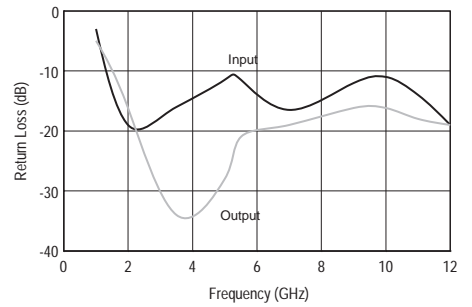
Return Loss
