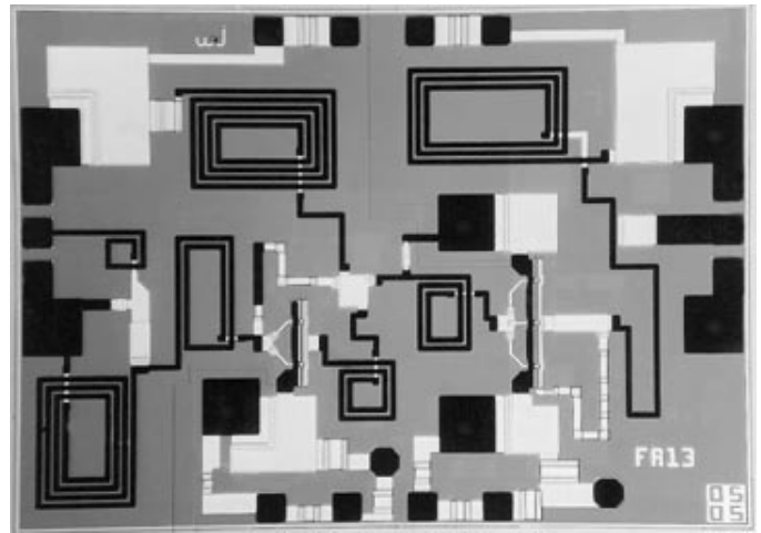
ICA1009 Chip Outline
