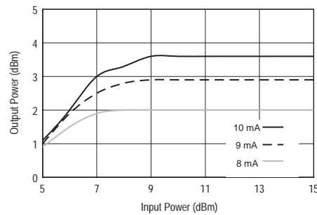
Max Limiting vs. Bias @ 12 GHz
