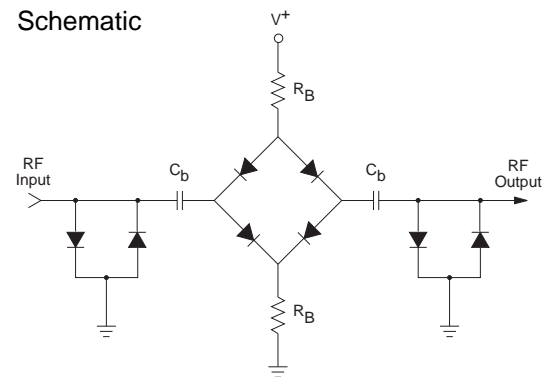
Assembly
