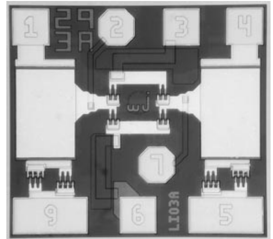
ICL1002 Chip Outline
