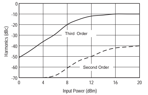
Harmonics @ 8 GHz
