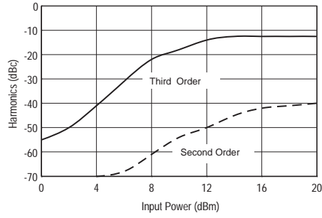
Harmonics @ 4 GHz
