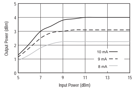
Max Limiting vs. Bias @ 8 GHz
