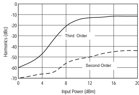
Harmonics @ 2 GHz
