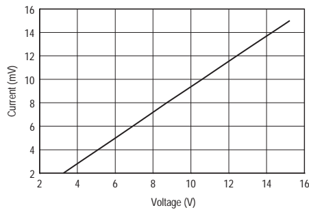
Bias Current vs. Voltage
