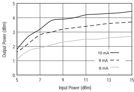
Max Limiting vs. Bias @ 2 GHz
