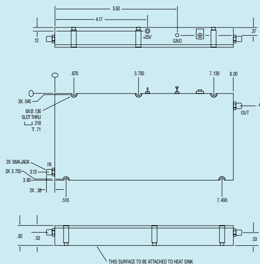
OUTLINE DRAWING
