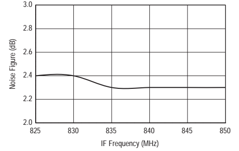
NF vs. IF Frequency @ +70°C
