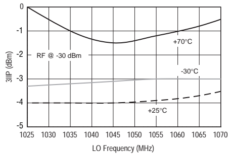
3IIP vs. LO Frequency
