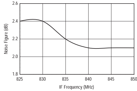
NF vs. IF Frequency @ +25°C
