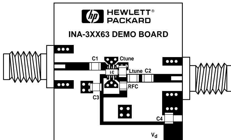
Figure 14. Assembled Amplifier.
