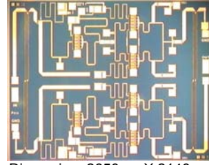
Dimension: 2650um X 2140um Thickness: 85um ± 15um
