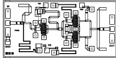
Dimension: 2250um X 1130um
