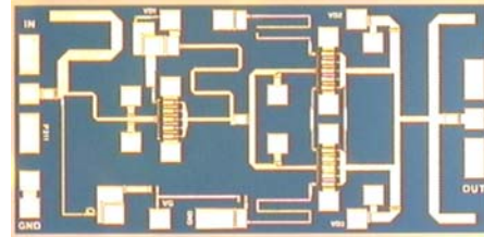
Dimension: 1130um X 2250um Thickness: 75um ± 13um
