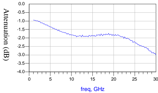
INSERTION LOSS
