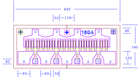
Chip Thickness: 75 ± 13 microns All Dimensions In Microns
