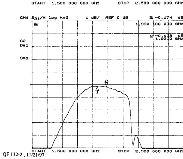
INSERTION LOSS
