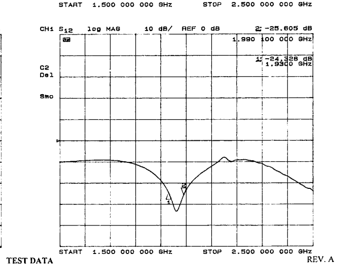
ISOLATION
