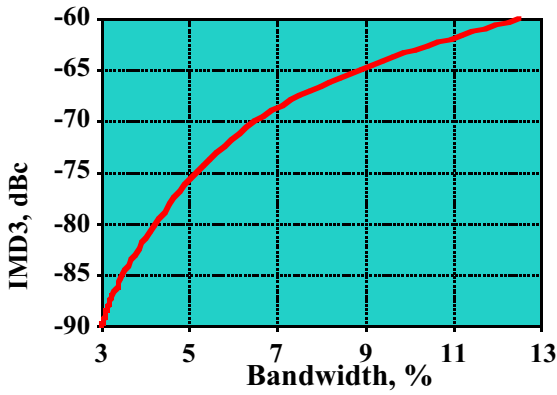
IMD PERFORMANCE
