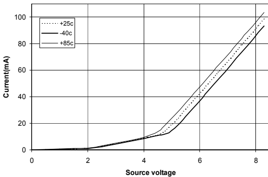
Bias Sweep vs. Temperature
