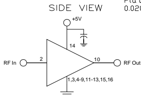
Application circuit
