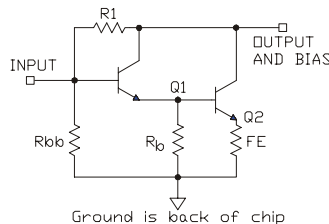
Simplified Schematic of MMIC
