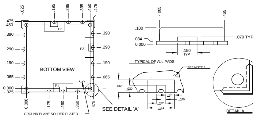
PHYSICAL DIMENSIONS
